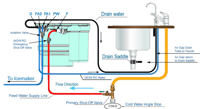
Figure 1: Installation Diagram
